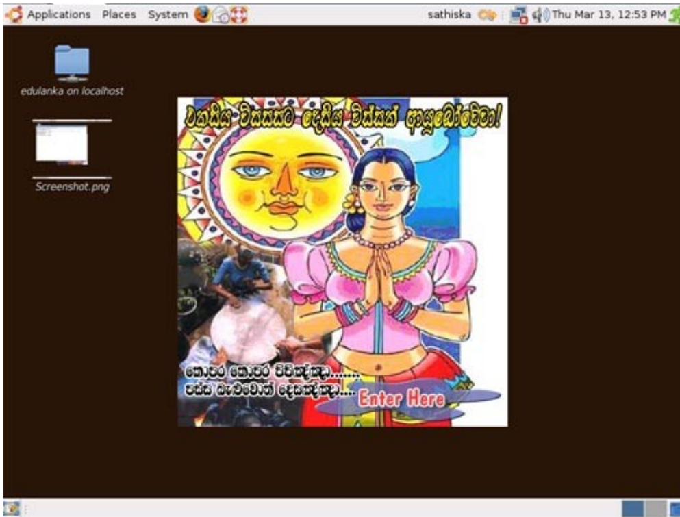
Edubuntu Desktop
